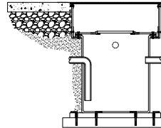
+ TAF Tank Anchor Flange
