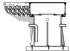
+ RAF Reinforcing Anchor Flange
